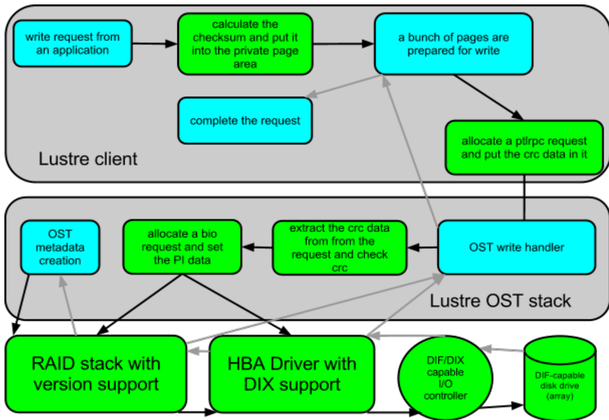
Figure 1. Flow of control on the write path. New or significantly changed SW/HW components are marked with green.
