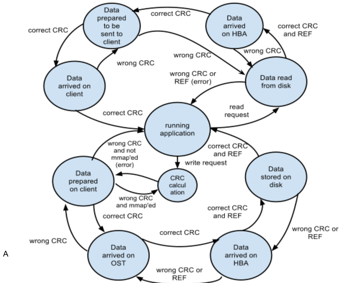
simplified verification-centric state diagram of Lustre end-to-end data integrity
