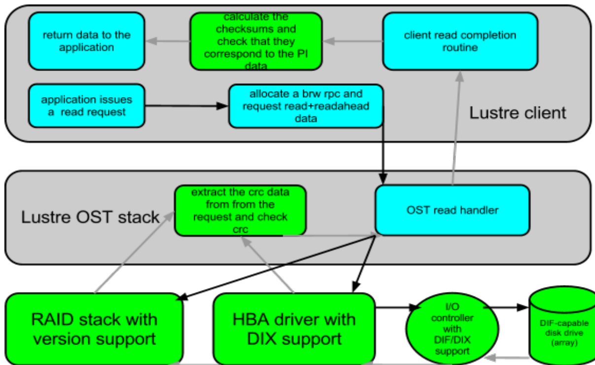
Figure 2. Flow of control on the read path. New or significantly changed SW/HW components are marked with green.
